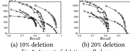
Fig. 9. Impact of deletion on Redcaps.
