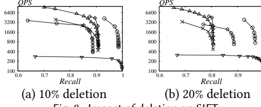
Fig. 8. Impact of deletion on SIFT.
