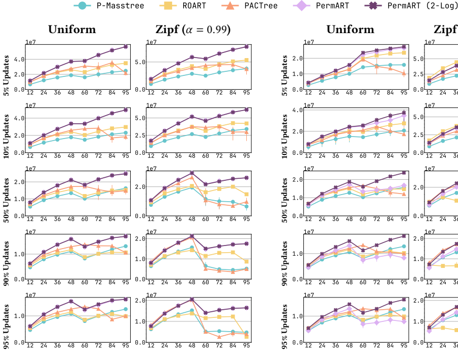
Fig. 5. Point operation performance in dense [1, 300M] universe prefilled to 100M. X: # threads. Y: ops/sec.
