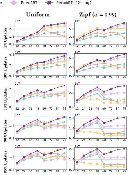
Fig. 6. Point operation performance in sparse [300M] universe of 64-bit keys prefilled to 100M. X: # threads. Y: ops/sec.
