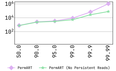
Fig. 13. Latency percentiles of \text{find}(\text{key}) operations. X: percentile. Y(\log) : Latency.
