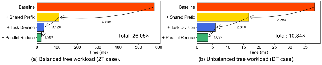
Fig. 9. Ablation Study.
