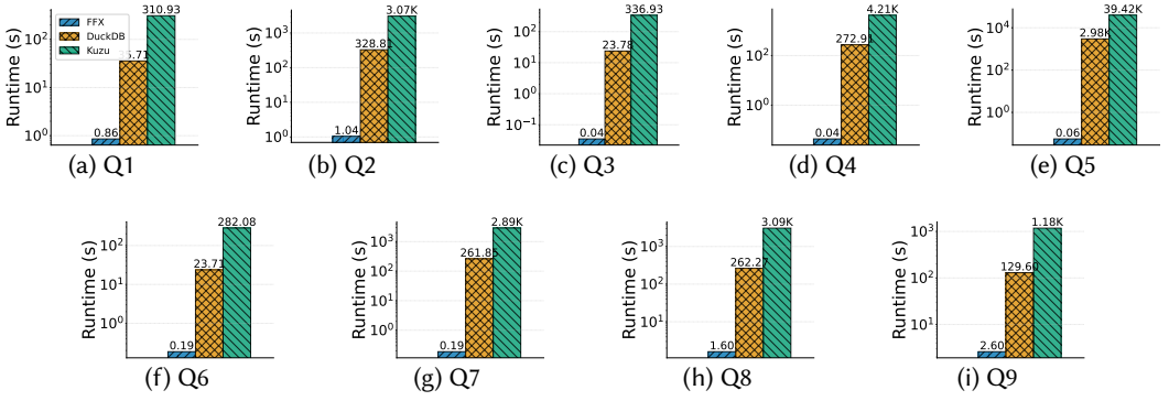
Fig. 9. Comparison of FFX, DuckDB, and Kuzu on Amazon for all nine queries, from Q1 to Q9, with MIN aggregation. Each system is run in single-threaded mode. FFX achieves speedsups: 10^2 – 10^5 × across queries.
