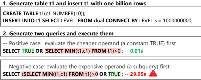
Fig. 1. A missed optimization detected by SCor in Oracle 23ai that leads to a 2995× performance degradation.
