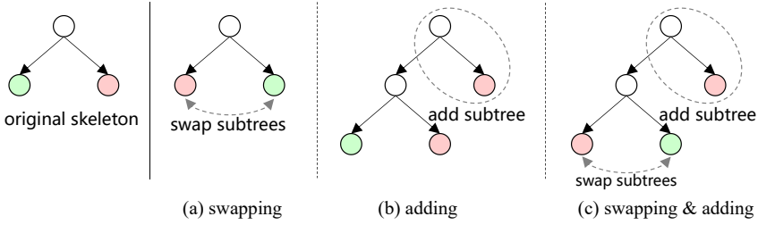
Fig. 3. Three transformation strategies used by SCor for modifying unbalanced short-circuit query skeletons in Table 1, including: (a) swapping, (b) adding, and (c) swapping & adding. ○ represents operators such as OR, AND, JOIN, INTERSECT; ● represents low-cost items, e.g., $lowCostTrueExpr , $lowCostEmptyStmt ; ● represents high-cost items, e.g., $highCostBoolExpr , $highCostStmt .
