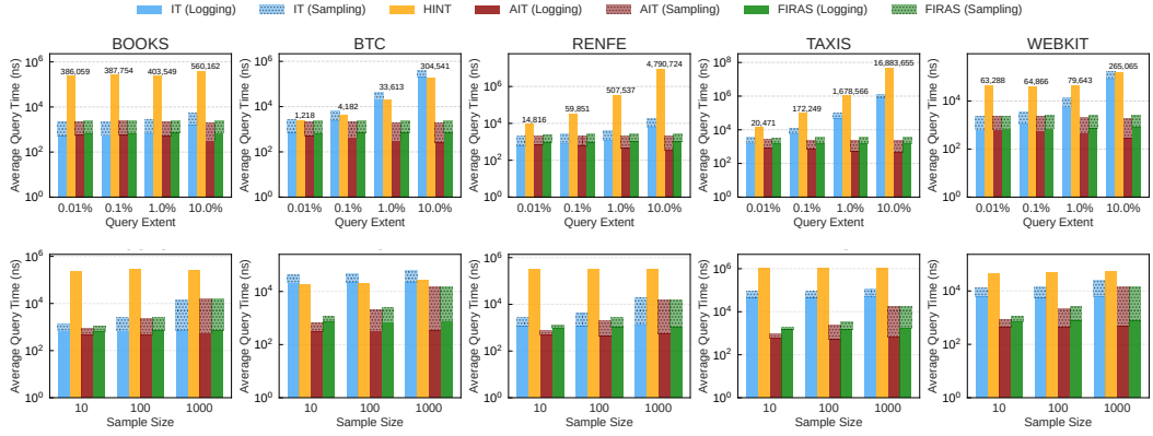
Fig. 7. Static data case, independent range sampling (the default query extent and sample size are respectively 1% and 100). Numbers over the bars are equal to the average size of a query result.
