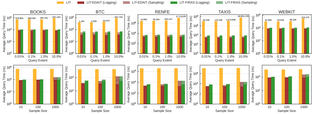
Fig. 10. Evolving data case, independent range sampling (the default query extent and sample size are respectively 1% and 100). Numbers over the bars equal to the average size of a query result.
