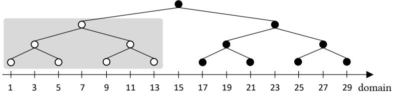
Fig. 4. Example of adding nodes to the EDIT. The nodes in the shadow are existing ones, whereas black nodes are newly added when D = 15 .
