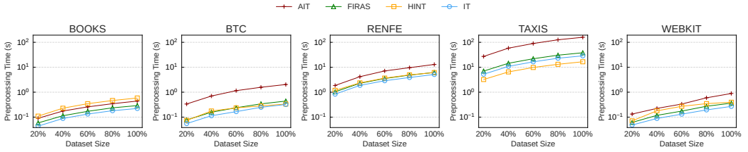
Fig. 5. Indexing time varying dataset size
