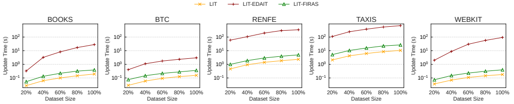
Fig. 8. Cumulative update time for evolving X
