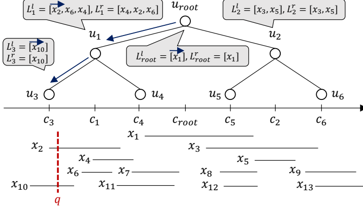
Fig. 1. Example of an interval tree and a stabbing query q . Because q < c_{root} , we access L_{root}^l , find that no interval is stabbed by q , and traverse its left child node u_1 . Because q < c_1 , we sequentially access the intervals \in L_1^l . We terminate the scan when x_6 is accessed because q < x_6.l . Next, we traverse its left child node u_3 and repeat the same sequential scan. Because u_3 is a leaf node, we return R = \{x_2, x_{10}\} .
