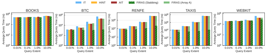
Fig. 6. Static data case, range query: FIRAS (Stabbing) and FIRAS (Array A) represent the times for stabbing query processing on IT and 1D range query processing on the sorted array \mathcal{A} , respectively.
