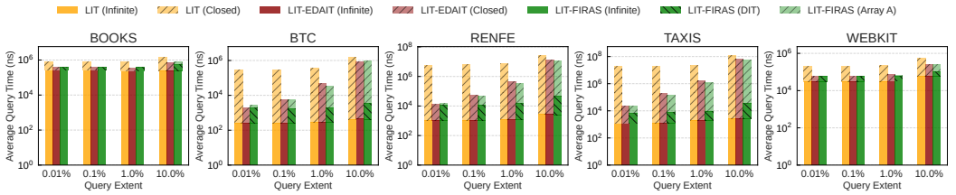
Fig. 9. Evolving data case, range query
