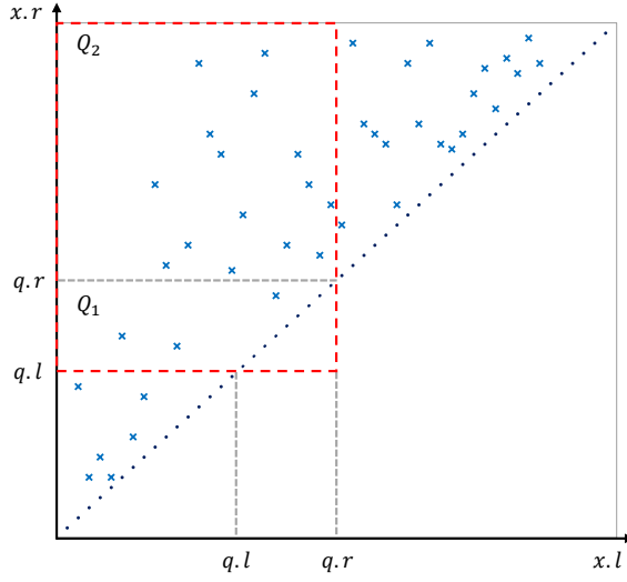
Fig. 2. Illustration of Proposition 3.1. Each interval x is transformed to a 2D point (represented as \times ) whose coordinates are (x.l, x.r) . A given query interval q is transformed into a two-sided orthogonal range query (-\infty, q.r] \times [q.l, \infty) shown as a dashed rectangle. The query rectangle can be split into a 1D range query in the x.r domain ( Q_1 ) and a stabbing query ( Q_2 ) on the intervals.
