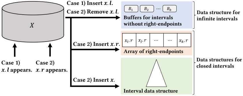
Fig. 3. Example of FIRAS for evolving X and how to deal with endpoint insertions. A sequence of buffers is used to manage open-ended intervals, whereas closed intervals are maintained with a sorted array and an interval data structure similar to FIRAS for static interval data.
