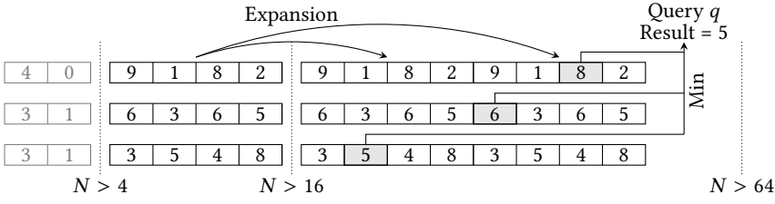
Fig. 7. Sublime CMS expands by concatenating each array with a copy of itself. It maps a key to a counter in an array by taking the appropriate number of bits from its hash.
