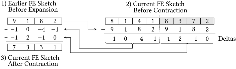
Fig. 8. During contractions, Sublime CMS extracts the recent updates by subtracting the previous FE sketch. It adds the results to the previous sketch to transfer the updates.
