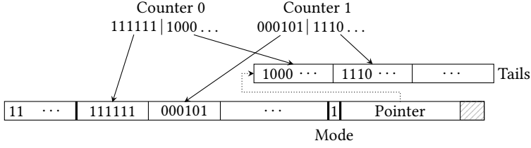
Fig. 6. When a chunk's extensions outgrow its space, it stores a pointer to a dedicated external array of tails to store the counters' higher-order bits.
