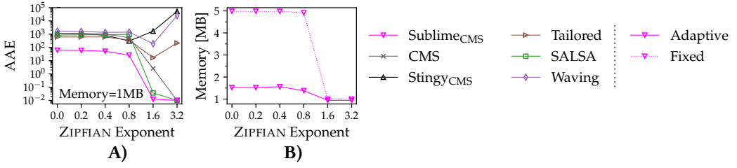
Fig. 11. By adapting VALE to skew, Sublime CMS achieves the highest accuracy among all baselines (Part A) and a smaller memory footprint compared to using a fixed tuning (Part B).
