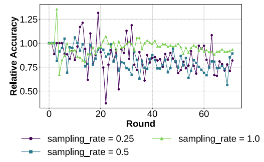
Fig. 15. Impact of sampling rate.
