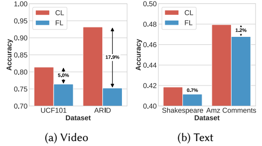
Fig. 9. CL and FL on naturally noisy datasets.
