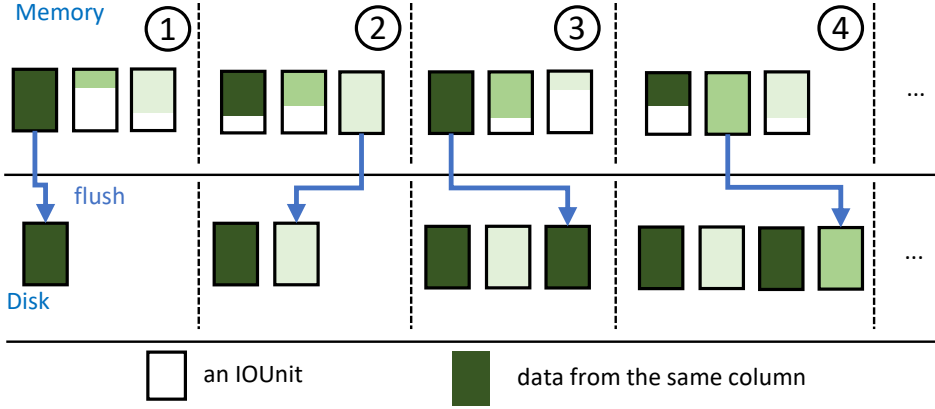
Fig. 4. F3's Writing Process – Different color means data from different columns. F3 flushes an IOUnit to disk as long as the column writer buffers enough data in memory. Parquet, on the other hand, must buffers the entire row group. The column chunk sizes thereby vary significantly, leading to non-optimal I/O sizes.
