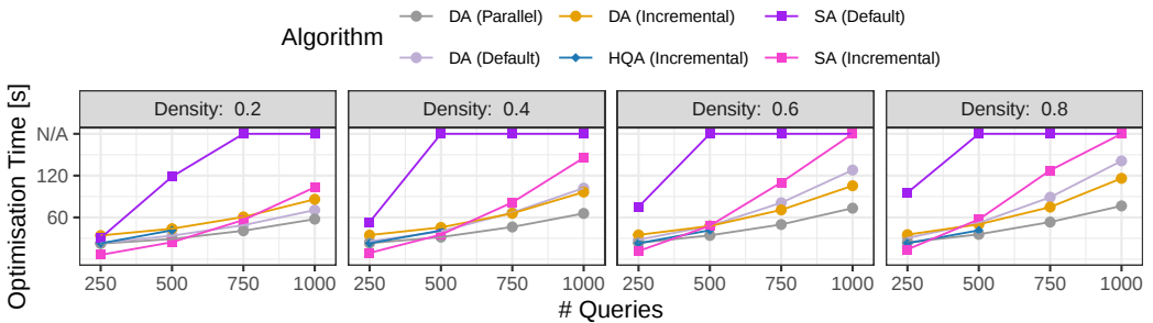
Fig. 7. Optimisation times for various MQO algorithms, yielded for MQO problems featuring increasing numbers of queries, 30 PPQ, as well as increasing savings densities. Cases where no result is obtained before 180s are labeled by N/A.
