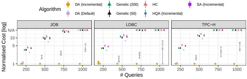
Fig. 6. Normalised solution costs for problems with 30 PPQ and increasing numbers of queries (cf. Fig. 3 for details).
