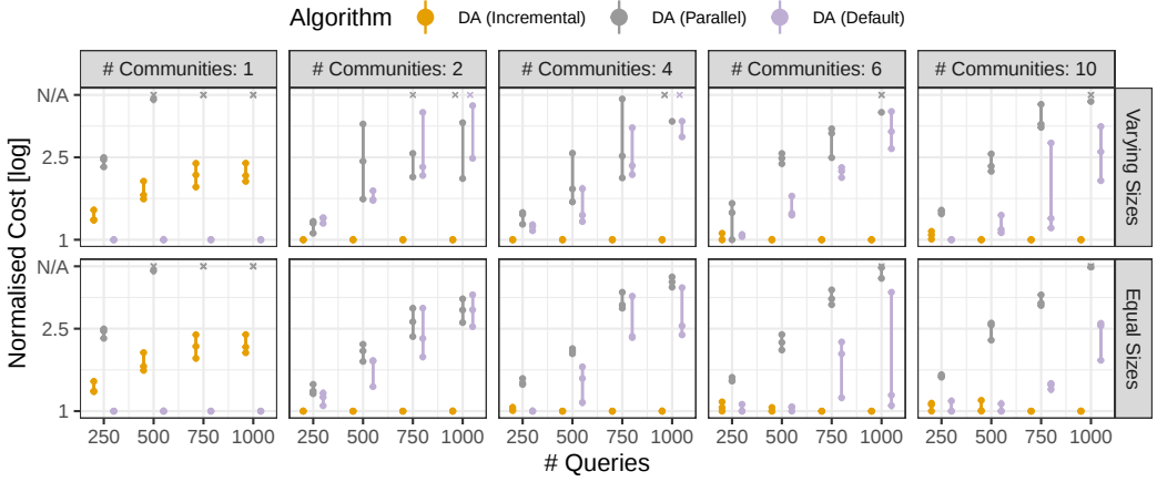
Fig. 4. Normalised solution costs for problems with 30 PPQ for varying numbers of queries and query communities; community densities are sampled from [0.05, 1] . Instances exhibit varying (top row) and equal (bottom row) community sizes. Costs \geq 5 are mapped to N/A; other details follow the presentation in Fig. 3.
