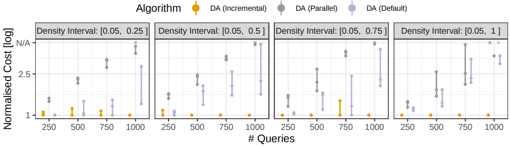
Fig. 5. Normalised solution costs for problems with 30 PPQ and increasing numbers of queries, and four query communities of varying sizes. Community densities are sampled from increasing intervals (cf. Fig. 3 for details; costs \geq 5 mapped to N/A).
