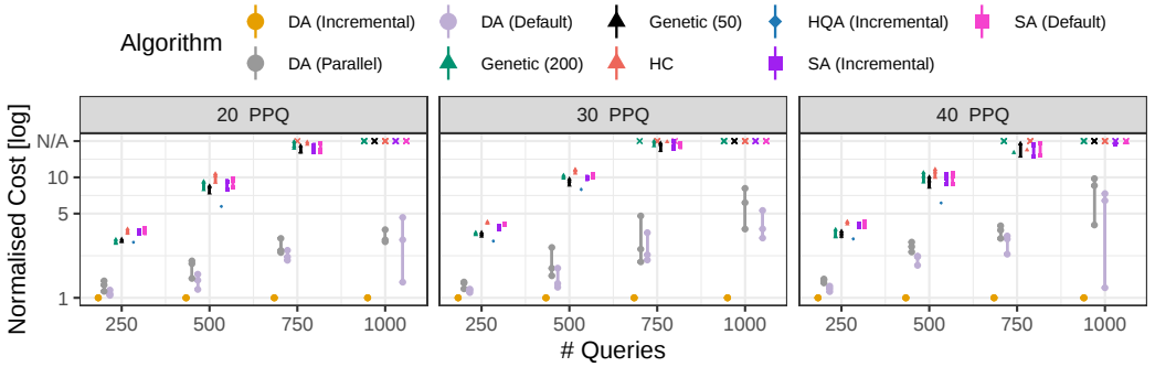
Fig. 3. Normalised solution costs (relative to overall best solutions) for instances with varying amounts of queries and plans per query (PPQ), and four query communities of varying sizes. We sample community densities from [0.05, 1] . Range lines visualise minimal and maximal normalised costs for a set of instances; individual solutions are given by small dots. Crosses with value N/A represent prohibitively large costs \geq 20 (slightly jittered horizontally and vertically to resolve outlier count).
