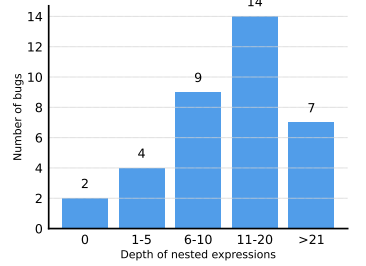
Fig. 15. Distribution of bugs based on the depth of nested expressions.
