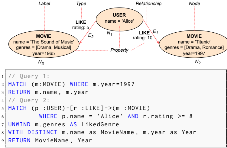
Fig. 2. An example labeled property graph storing the movies that users like (top) and two examples of Cypher queries retrieving movie's name and year (bottom).
