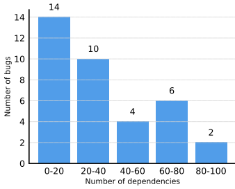
Fig. 13. Distribution of bugs based on the number of dependencies involved.
