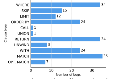
Fig. 12. The number of bugs related to different types of clauses.
