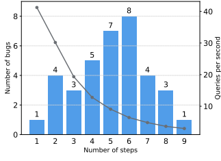
Fig. 10. Distribution of all 36 bugs across the tested databases, categorized by the different synthesis steps involved.
