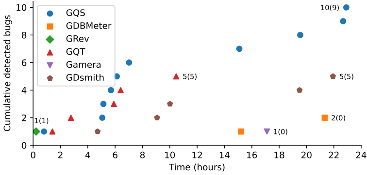
Fig. 18. Cumulative bugs detected in Neo4j and FalkorDB over 24 hours. We follow the same setup as in Table 6.
