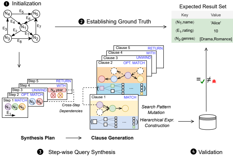
Fig. 3. The workflow of GQS.
