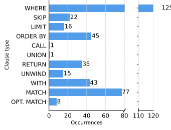
Fig. 11. The aggregated number of clauses involved in the bug-triggering test queries.
