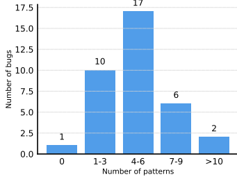
Fig. 14. Distribution of bugs based on the number of patterns involved.
