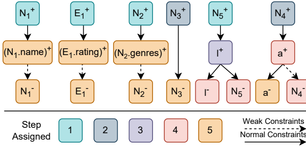
Fig. 4. An illustration of assigning operations across different steps based on Example 3.2.
