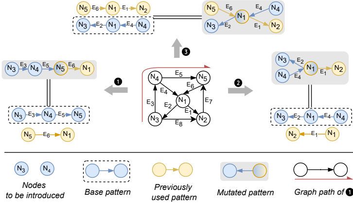
Fig. 5. Three pattern mutation strategies.
