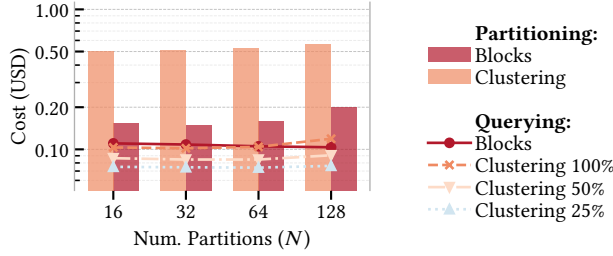
Fig. 9. Total indexing and querying costs of clustering-based and block-based data partitioning with 10 batches of 5000 queries (DEEP10M dataset).
