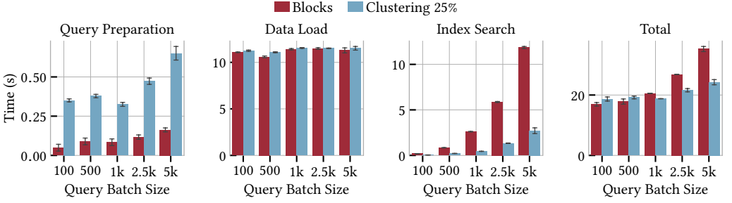
Fig. 8. Querying time comparison of block-based versus clustering-based ( N_{\text{search}} = 25\% ) data partitioning for different query batch sizes, using the DEEP10M dataset with 32 partitions. Besides the three phases shown, the total time includes function invocation overhead and the reduction operation, which vary minimally and, aggregated, add \approx 6 s on average.
