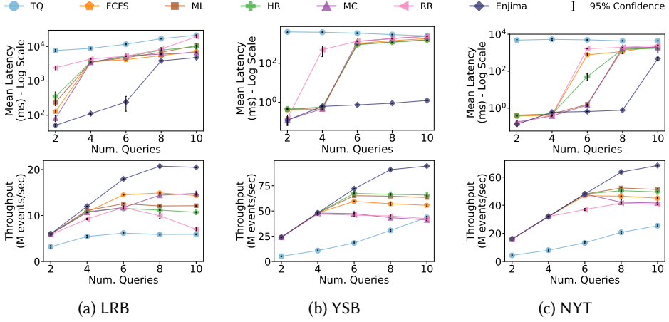
Fig. 5. Performance of scheduling policies for LRB, YSB, and NYT benchmarks
