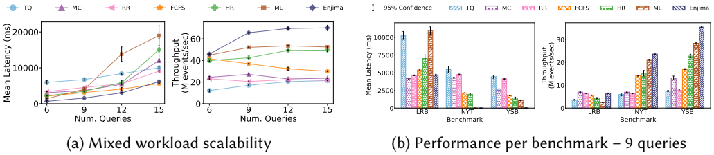
Fig. 8. Performance of scheduling policies for a heterogeneous mix of LRB, YSB, and NYT
