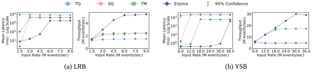
Fig. 9. Performance for single LRB and YSB queries
