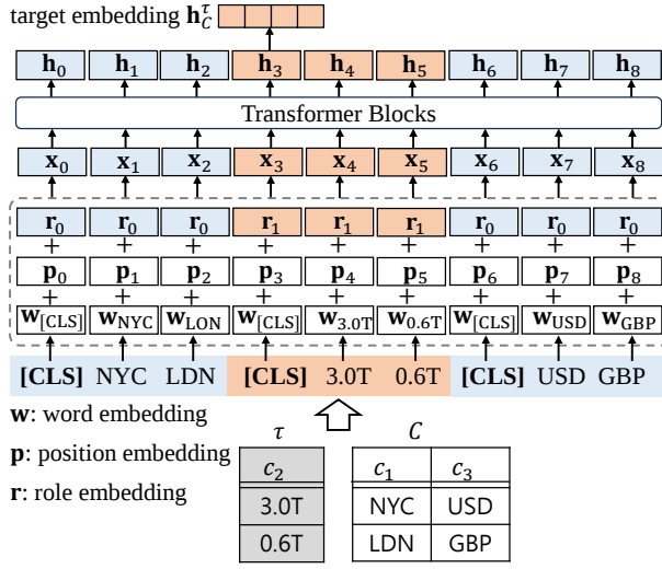
Fig. 4. Illustration of Context-Aware Column Embedding.
