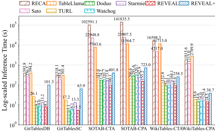
Fig. 6. Inference time comparison.
