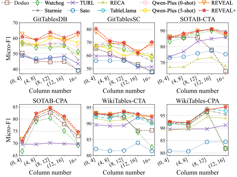
Fig. 5. Performance on tables with a small to large number of columns.
