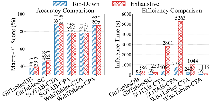
Fig. 7. Comparison between the Top-Down inference strategy and Exhaustive search in terms of accuracy (Macro-F1) and inference efficiency.
