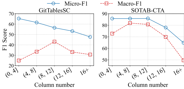
Fig. 2. The impact of column number on CTA.
