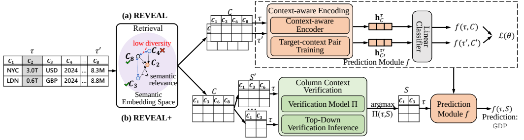
Fig. 3. The Framework of REVEAL and REVEAL+.
