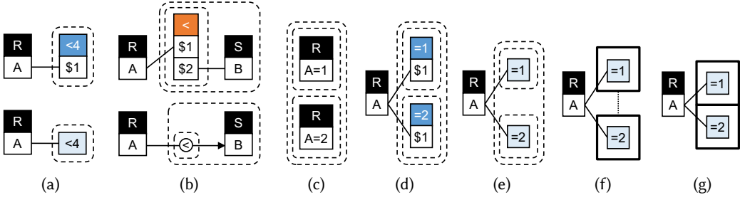
Fig. 6. Example 6(a-b) : Representation B at the bottom, and Relational Diagrams with anchor relations at the top. Example 7 (c-g) : \exists r \in R[r.A=1 \vee r.A=2] : (c): Relational Diagrams. (d): Relational Diagrams with anchor relations . (e-g): Representation B. (f-g) show our visual shortcut for disjunctions, formally justified with what we refer to as “De Morgan-fuse boxes”.
