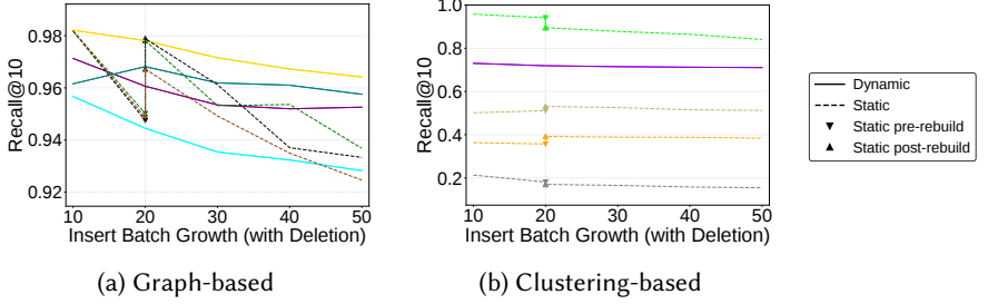
Fig. 11. Static vs. Dynamic under Streaming Inserts with Deletions
