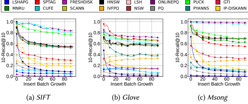
Fig. 3. Continuous Recall vs. Insert Batch Growth
