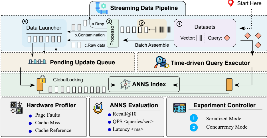
Fig. 1. Open-world ANNS benchmark flowchart
