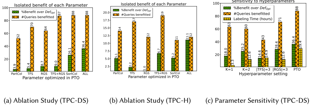
Fig. 9. Isolated Benefit of Each Parameter (Ablation Study) and Sensitivity to Hyperparameters
