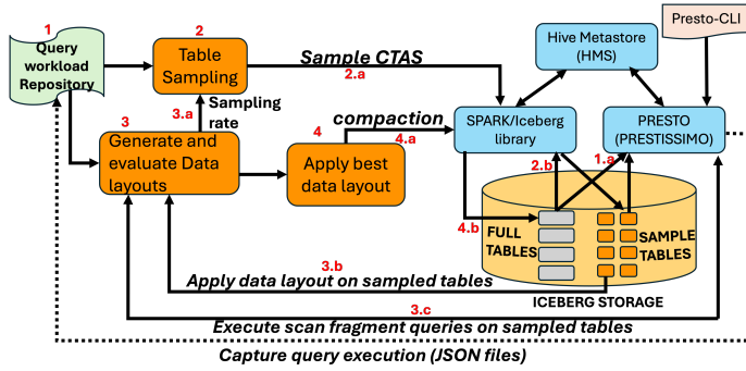
Fig. 1. System Architecture of PTO
