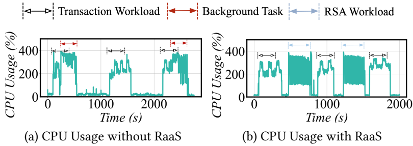
Fig. 10. CPU Usage
