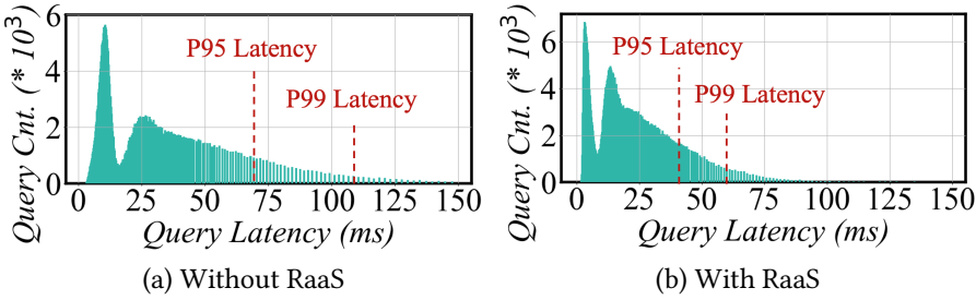
Fig. 9. Query Latency Distribution in Neon
