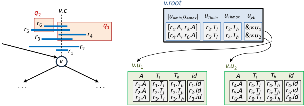
Fig. 5. The RISH index (right) of an AITTI node v (left) and two time-travel queries
