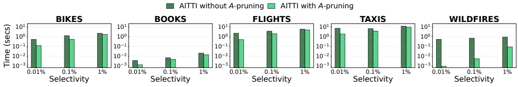
Fig. 8. Impact of A -attribute pruning on AITTI's total time while varying the query selectivity
