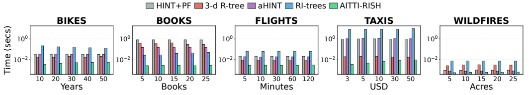
Fig. 13. AITTI-RISH against competition, total time for stabbing time-travel queries while varying A-range query extent
