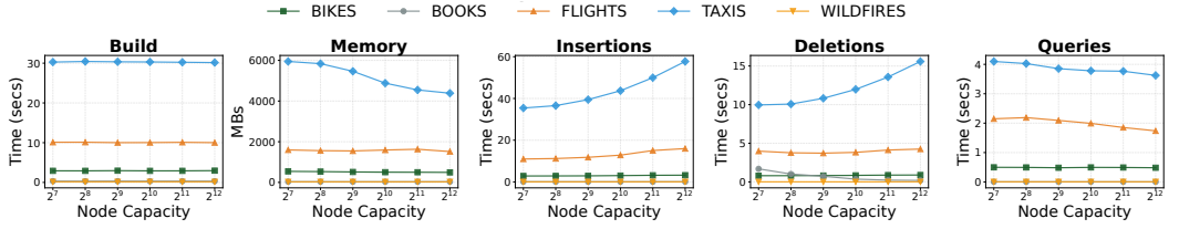
Fig. 7. Impact of RISH's node capacity on AITTI; time-travel queries with a fixed query selectivity of 0.1%
