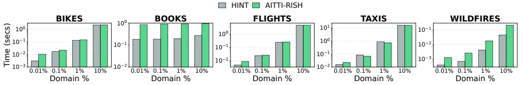
Fig. 14. AITTI-RISH against competition, total time for time-only queries while varying query extent
