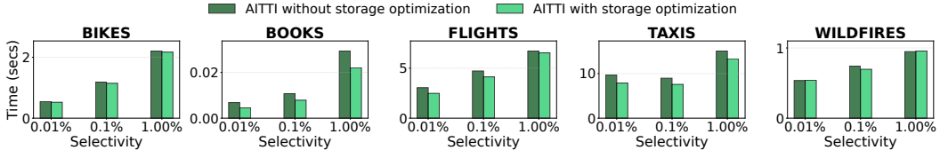
Fig. 6. Impact of storage optimization on AITTI's total time while varying the query selectivity; RISH node capacity C = 128
