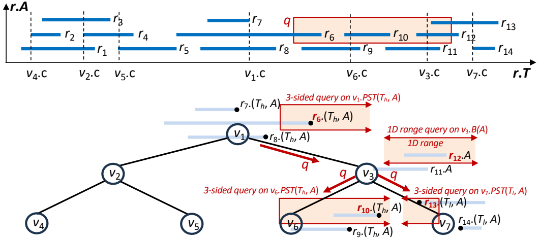
Fig. 4. An AITTI for temporal records and an exemplary query q , shown as a rectangle that models a combined temporal range with an attribute range filter. At each interval tree node accessed by the query, only the searched local data structures are shown.
