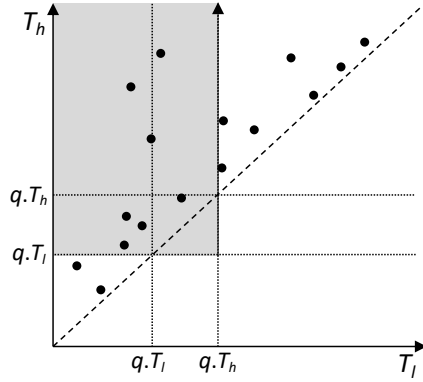
Fig. 10. Space transformation for the 3-d R-tree baseline
