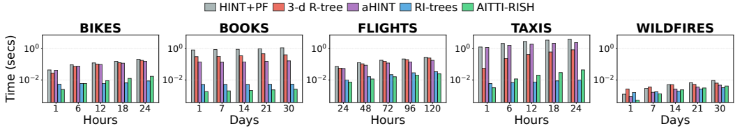
Fig. 12. AITTI-RISH against competition, total time for equality time-travel queries while varying time range query extent
