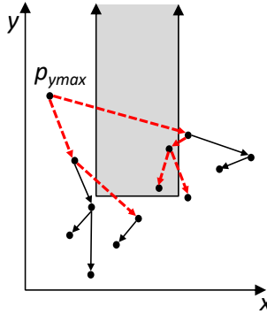
Fig. 3. Example of a priority search tree and 3-sided query
