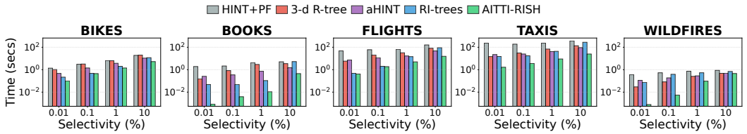
Fig. 11. AITTI-RISH against competition, total time for time-travel queries while varying query selectivity
