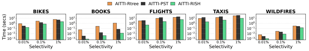
Fig. 9. Total time of AITTI variants for time-travel queries while varying the query selectivity
