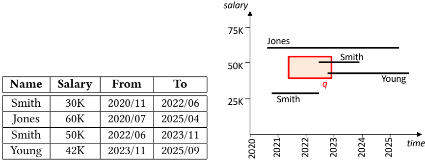
Fig. 1. A Temporal employee records (left); their geometric representation and a time-travel query (right)
