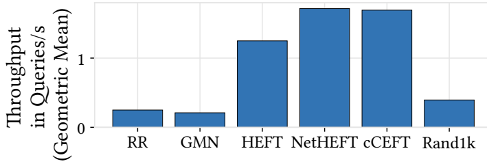
Fig. 15. Execution throughput of queries with growing intermediate results after 2x scale-out from small to large nodes.
