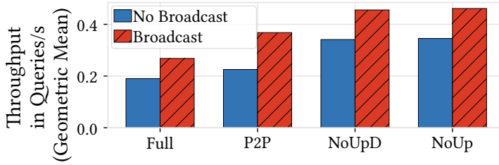
Fig. 6. Query throughput for variations of state separation across TPC-H, TPC-DS, and JOB.
