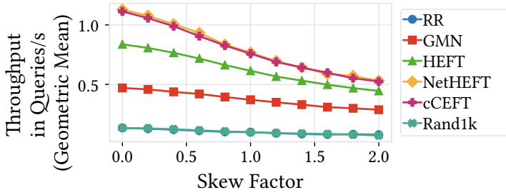
Fig. 17. Execution speed with increasing partition skew.
