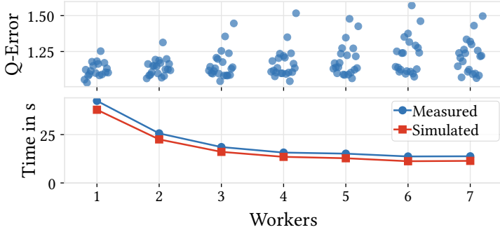
Fig. 8. Simulated and Trino execution of all TPC-H queries across varying numbers of workers.
