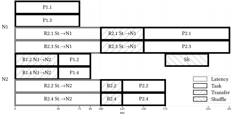
Fig. 4. Simulation timeline for running example.
