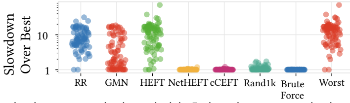
Fig. 16. Execution slowdown compared to best schedule. Each marker represents the slowdown on one query.
