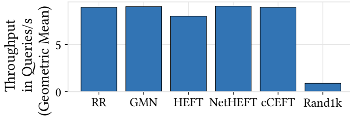
Fig. 11. Execution throughput in common scenario
