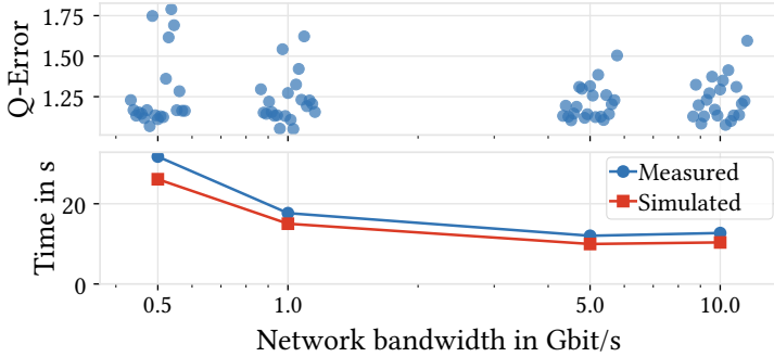
Fig. 9. Simulated and Trino execution of all TPC-H queries across varying network speeds.
