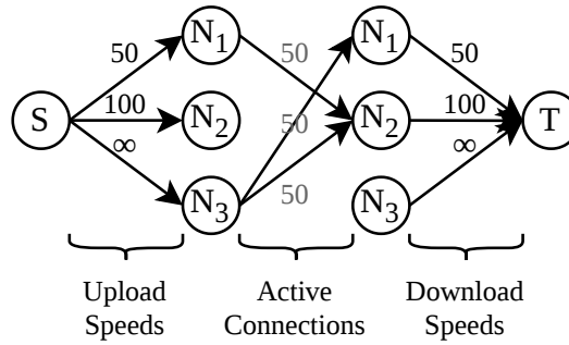
Fig. 5. Modeling the network throughput in Gbit/s of data streams as a max-flow problem.
