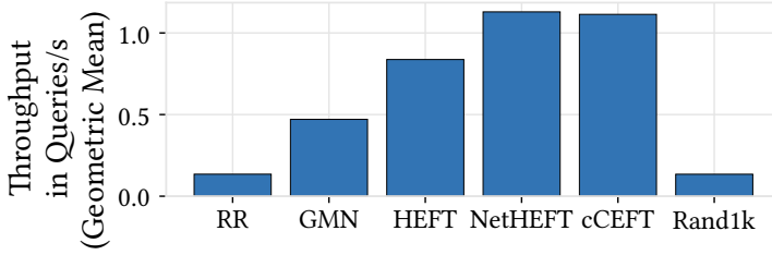
Fig. 13. Execution throughput after 2x scale-out from small to large nodes.
