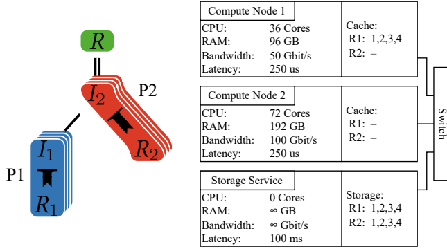
Fig. 1. A distributed query and the state of a cluster.
