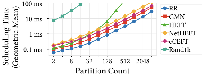
Fig. 19. Scheduling time for different partition counts.
