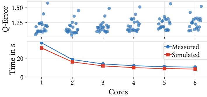
Fig. 10. Simulated and Trino execution of all TPC-H queries across varying worker sizes.
