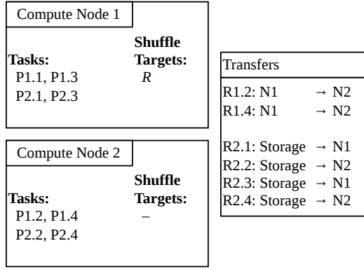
Fig. 2. Example of a possible assignment of tasks to nodes
