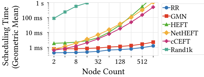
Fig. 20. Scheduling time for different node counts.
