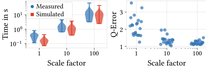
Fig. 7. Simulated execution of all TPC-H queries with different scale factors compared to Trino execution.
