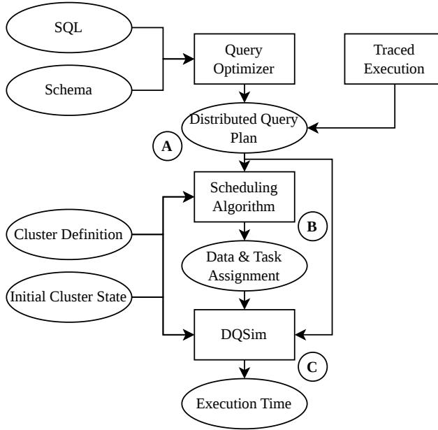
Fig. 3. Overview of the simulation workflow.
