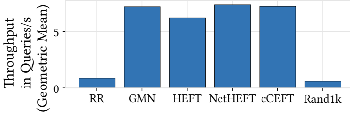
Fig. 12. Execution throughput after 2x scale-out.
