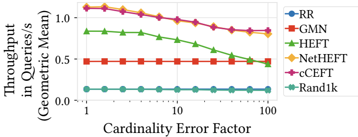
Fig. 18. Execution speed with increasing cardinality estimation errors.
