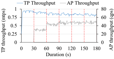
Fig. 12. Throughput with varying AP clients over time (SSB-TC Uniform).
