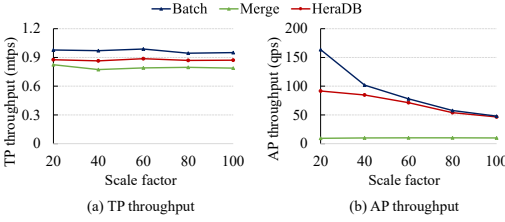
Fig. 14. Throughput with varying scale factors.
