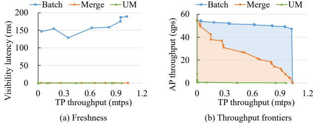
Fig. 3. Results of CPU-GPU HTAP execution strategies.
