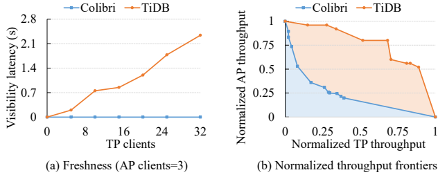
Fig. 2. Performance metrics across HTAP architectures.
