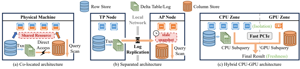
Fig. 1. Comparison of HTAP architectures. (a) Co-located: Low isolation due to CPU and memory resource contention. (b) Separated: Low freshness due to log propagation delay. (c) HeraDB: Achieves high freshness and strong isolation by offloading heavy scans to GPU while CPU handles lightweight delta updates.
