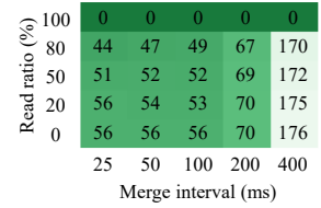
Fig. 18. Batch visibility latency with varying read ratios and merge intervals.
