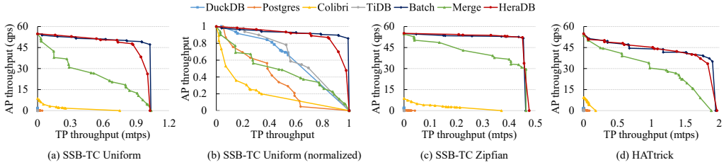
Fig. 10. Comparison of throughput frontiers (SF=100). Each frontier is constructed by connecting the best observed TP/AP throughput points from independent runs with different TP/AP client mixes.
