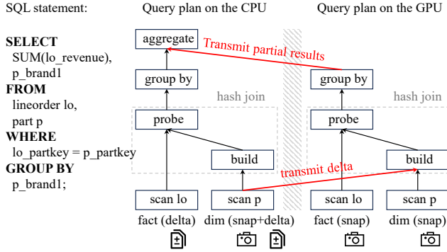
Fig. 8. An example of query result aggregation.
