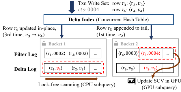
Fig. 5. Detailed design of the delta table.
