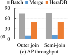
Fig. 13. Results of non-aggregatable query execution.
