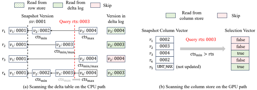
Fig. 6. An example of hybrid query execution.
