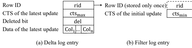
Fig. 7. Structure of the log entry in the delta table.
