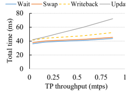
Fig. 15. Delta-merge latency breakdown.
