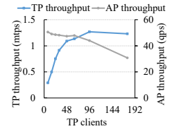
Fig. 16. Throughput varying TP clients across four NUMA nodes.
