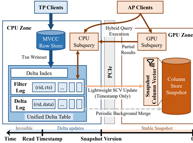
Fig. 4. System architecture and workflow.
