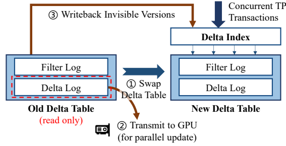
Fig. 9. Workflow of the delta merge process.
