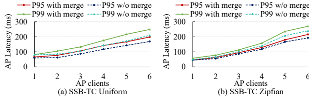
Fig. 11. AP query tail latency with varying AP clients.
