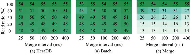
Fig. 17. AP throughput with varying read ratios and merge intervals.
