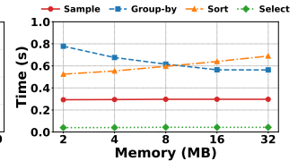
Fig. 14. Insertion time breakdown.
