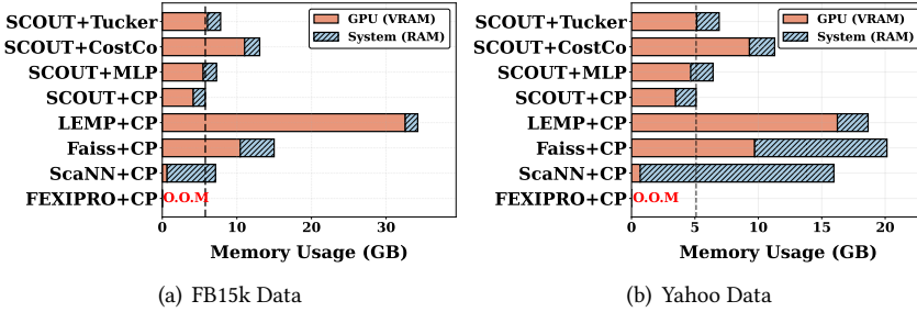
Fig. 4. Scout remains memory-efficient, whereas MIPS methods incur high memory cost or O.O.M. failures due to coupled materialization.
