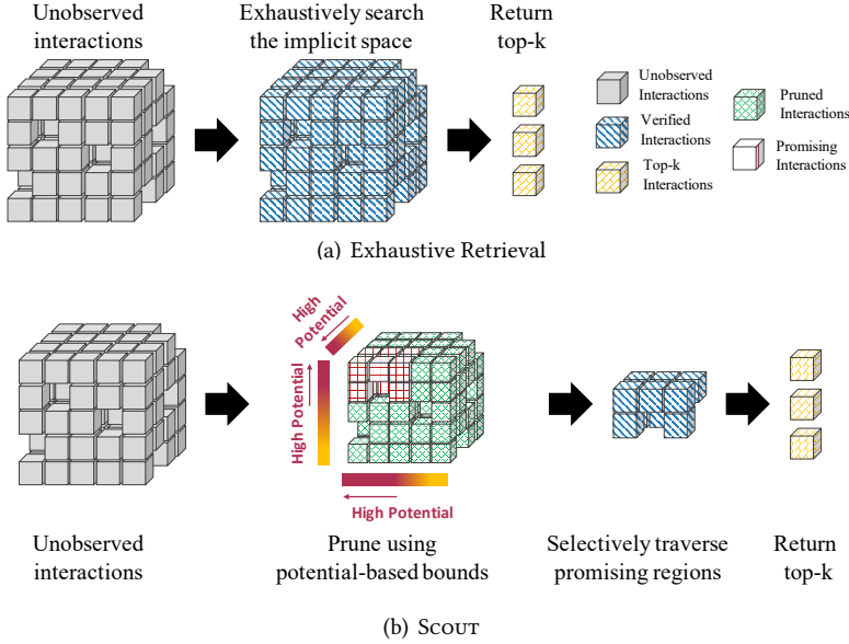
Fig. 1. Scalable top- k retrieval over implicit tensor spaces. Exhaustive retrieval requires searching the entire implicit interaction space, whereas Scout prunes unpromising regions and selectively verifies promising interactions.
