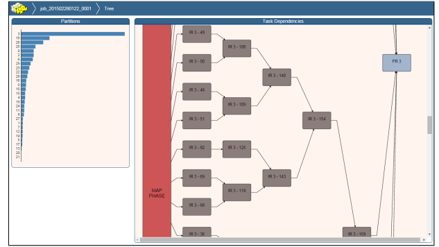
(b) Task dependencies in multiple iterations of IR phase
