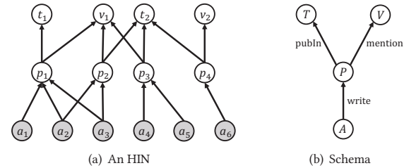
Figure 1: An example HIN with a star-schema.
