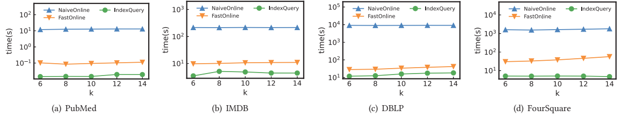
Figure 7: Efficiency results of three query algorithms.
