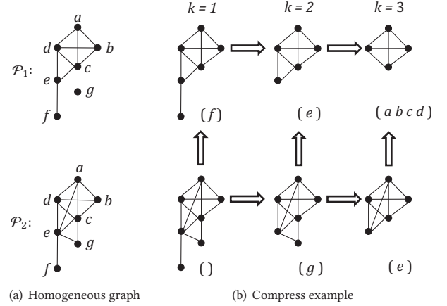
Figure 5: An example of MKC compression.
