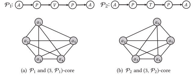
Figure 2: Induced homogeneous graphs of two communities.
