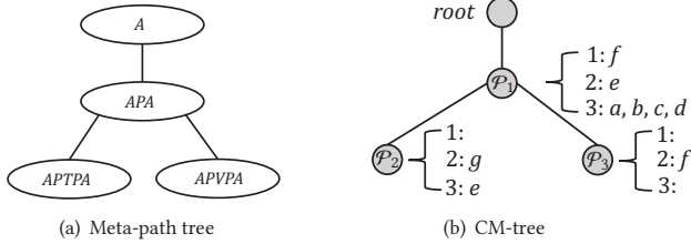
Figure 4: Meta-path tree and the corresponding CM-tree.
