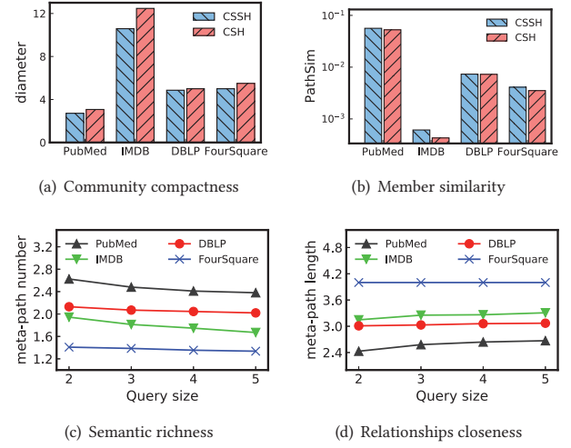
Figure 6: Results of effectiveness evaluation.
