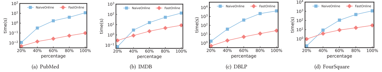
Figure 8: Scalability test for online query algorithms.
