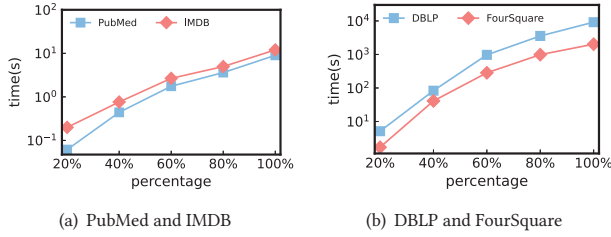
Figure 10: Efficiency results of index construction.
