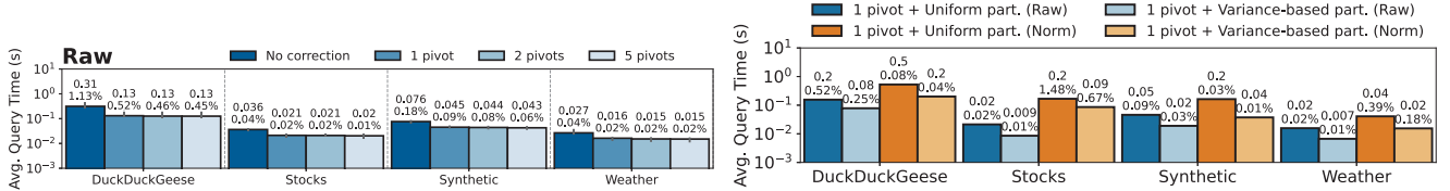
Figure 9: Impact analysis of the optimizations on MS-Index: (a) Query time over the number of pivots in DFT-bound correction; (b) Query time of weighted partitioning vs. uniform partitioning. Annotations indicate the average query time and the percentage of subsequences exhaustively considered (the rest is pruned).
